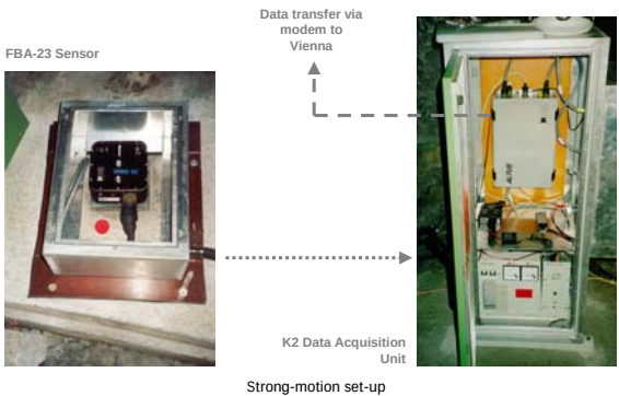
Strong-motion set-up
